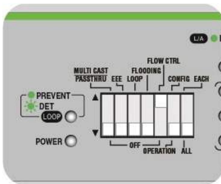
Figure 51. DIP Switch Settings for Enabling Flow Control
