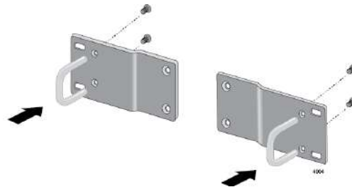
Figure 34. Attaching Handles to Brackets
